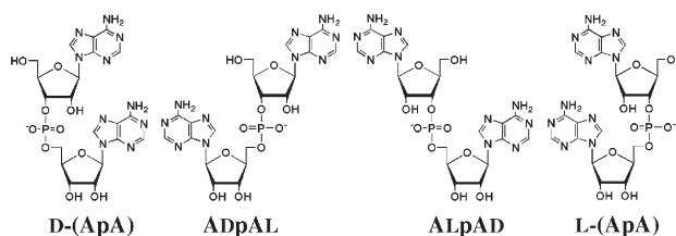
Fig. 1 Structures of diastereomeric ApAs.
